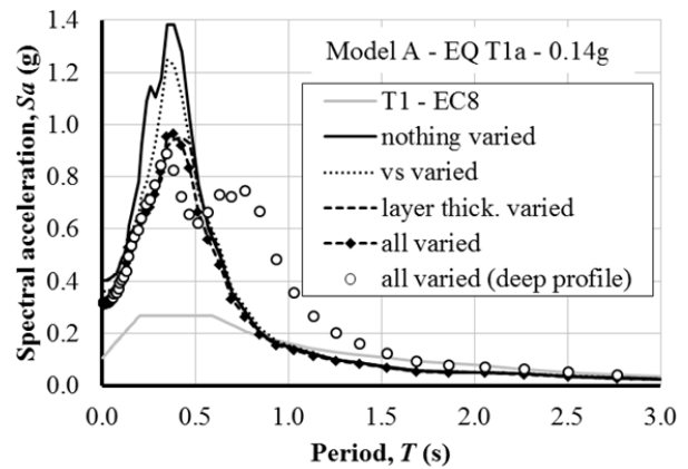
Fig. 11 Acceleration response spectra with parameter variations
